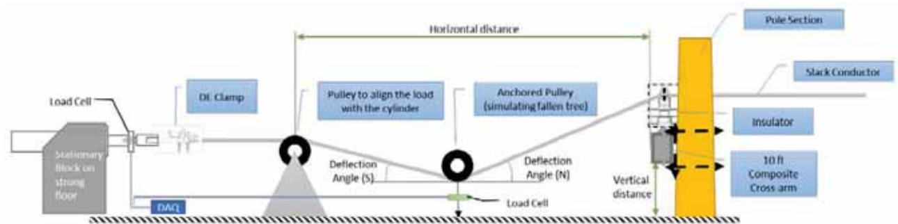
Figure 63. Schematic diagram of the full-system tree-fall test.
