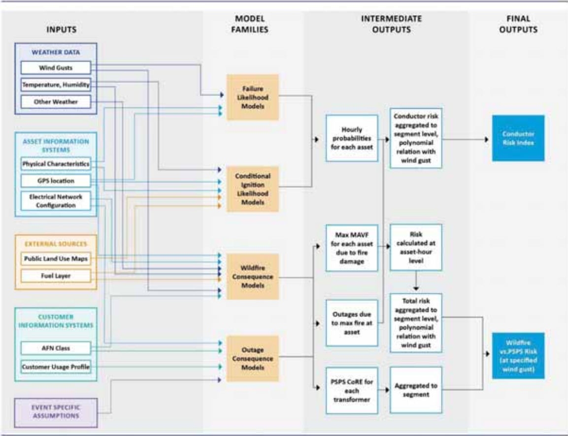
Figure 5: WiNGS-Ops Calculation Schematic
