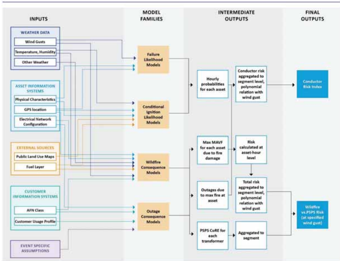
Figure 6-8: WiNGS-Ops Calculation Schematic
