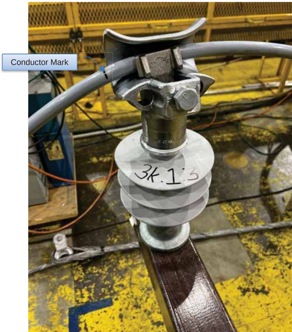
Figure 6-29: Sample 3K.1. – Insulator and Cross-arm Condition after Test
