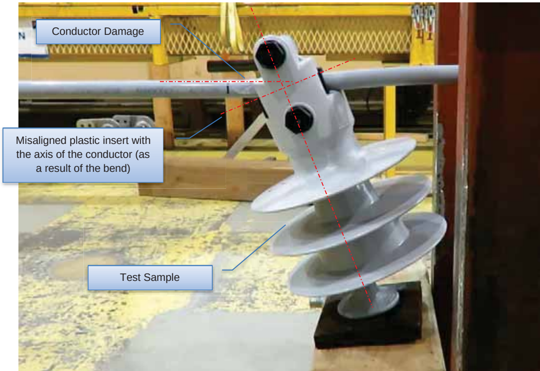
Figure 6-1: [REDACTED] - Typical Clamp and 1/0 AWG (17 kV) ACSR Conductor Position after Slip Test
