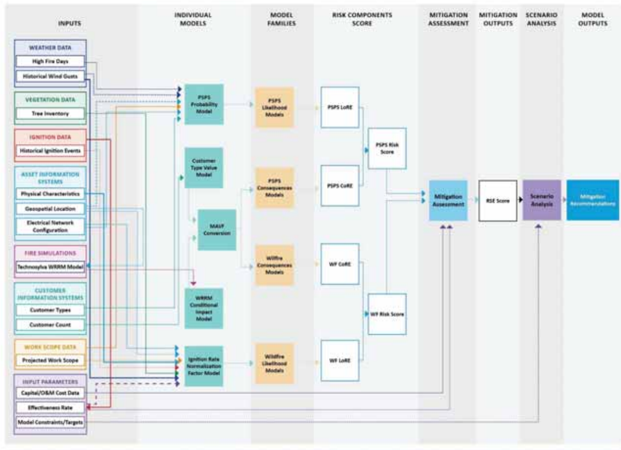
Figure 6-7: WiNGS-Planning Calculation Schematic
