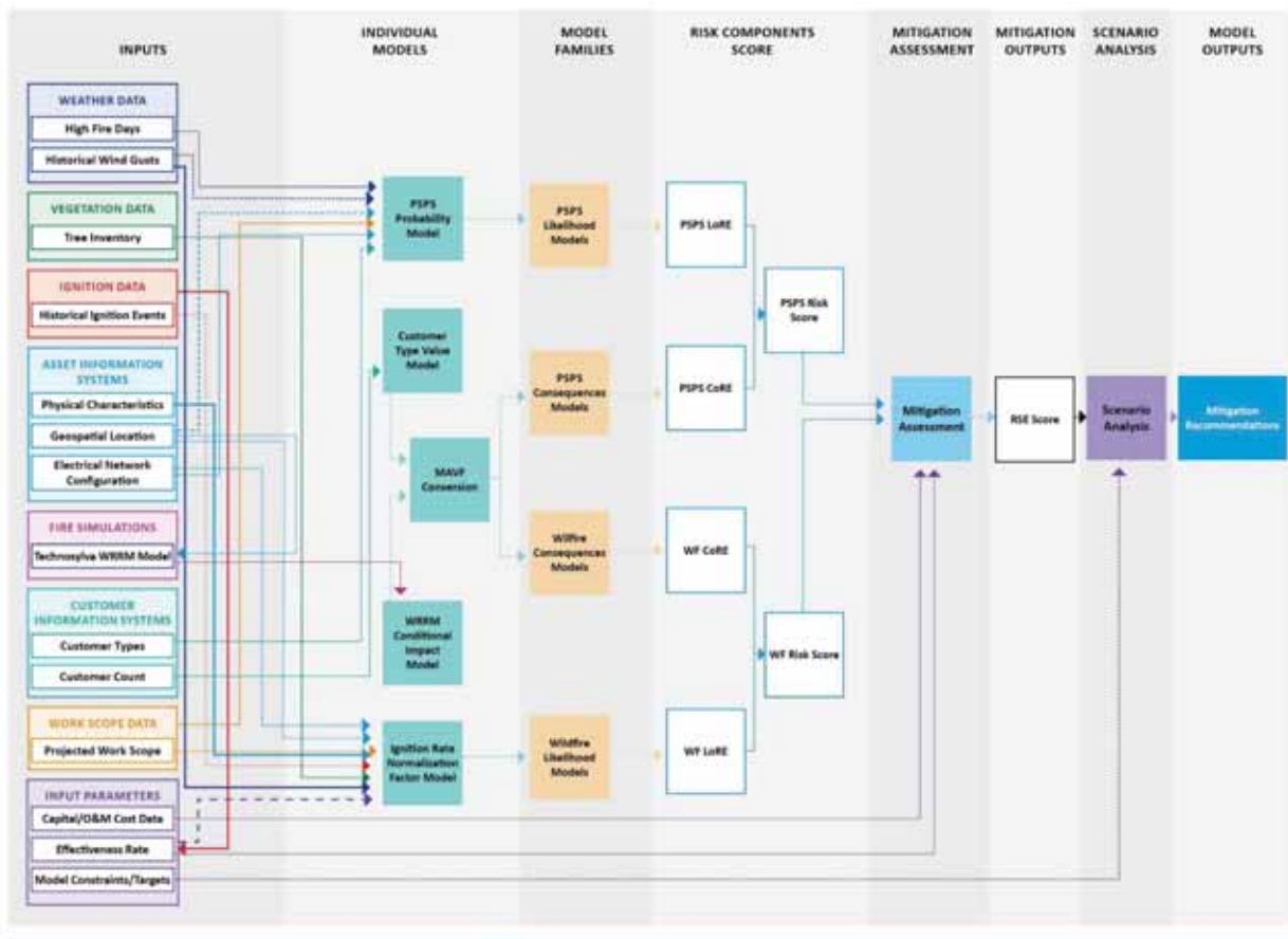
Figure 2: WINGS-Planning Calculation Schematic
