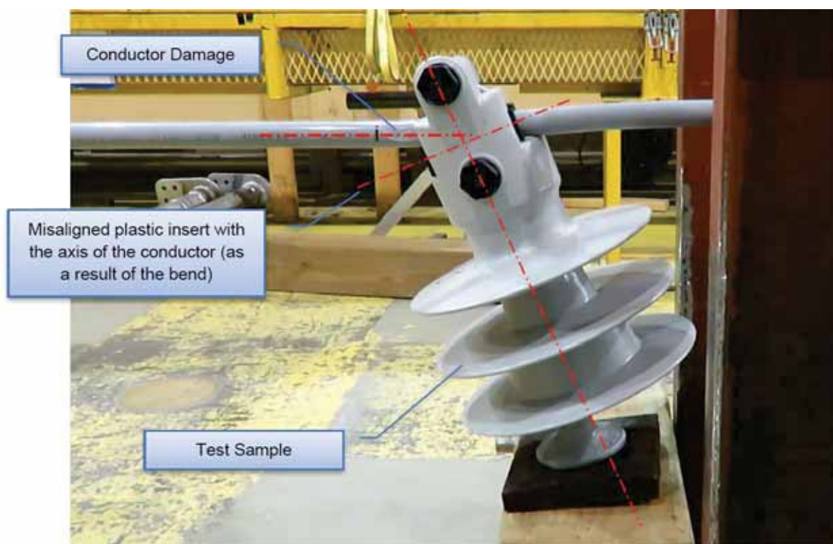
Figure 66. A representative post-test image of a vise-top insulator illustrating the bending behavior of the insulator that leads to conductor slippage (1/0 ACSR).
