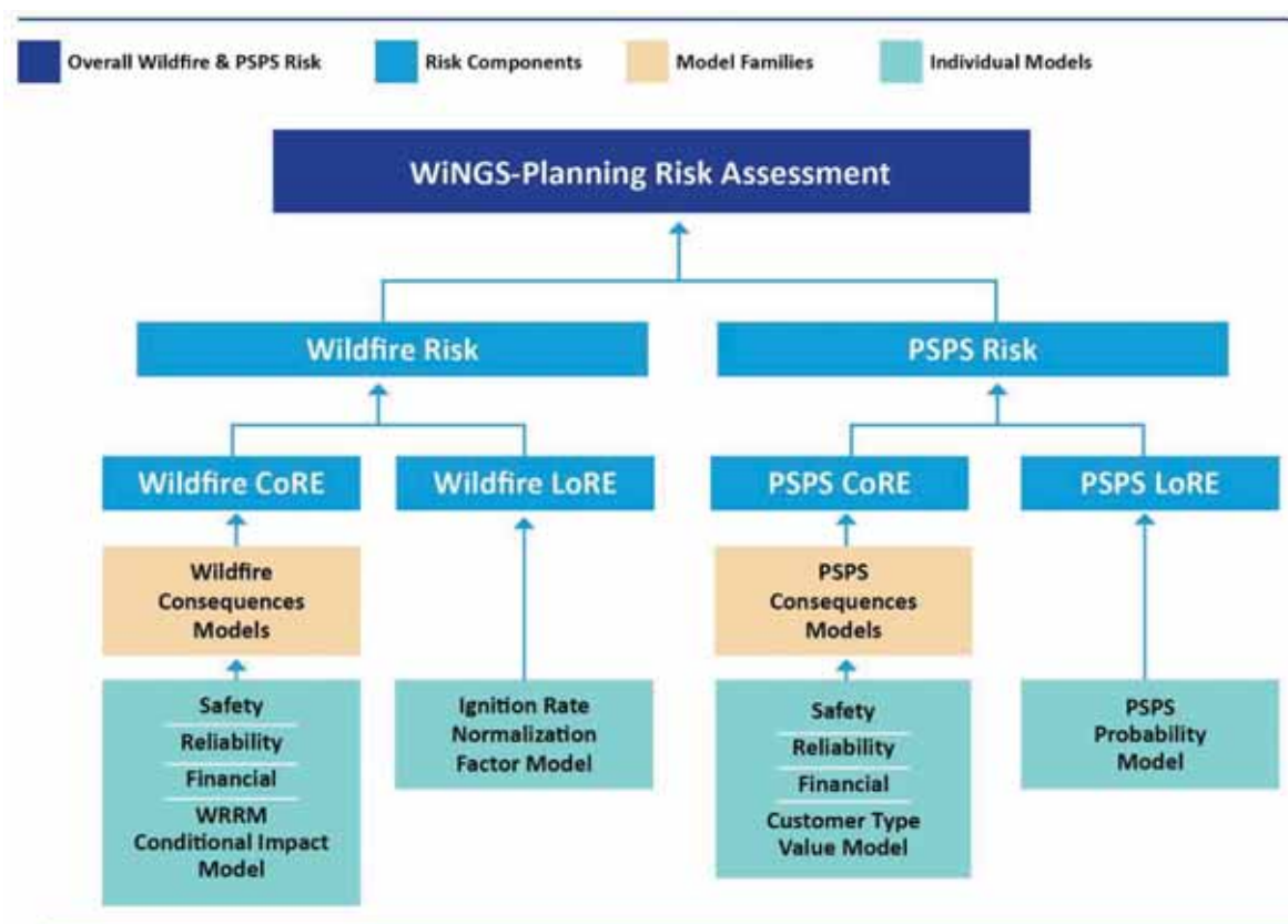
Figure 6-4: WiNGS-Planning Risk Calculation Process Flow Diagram
