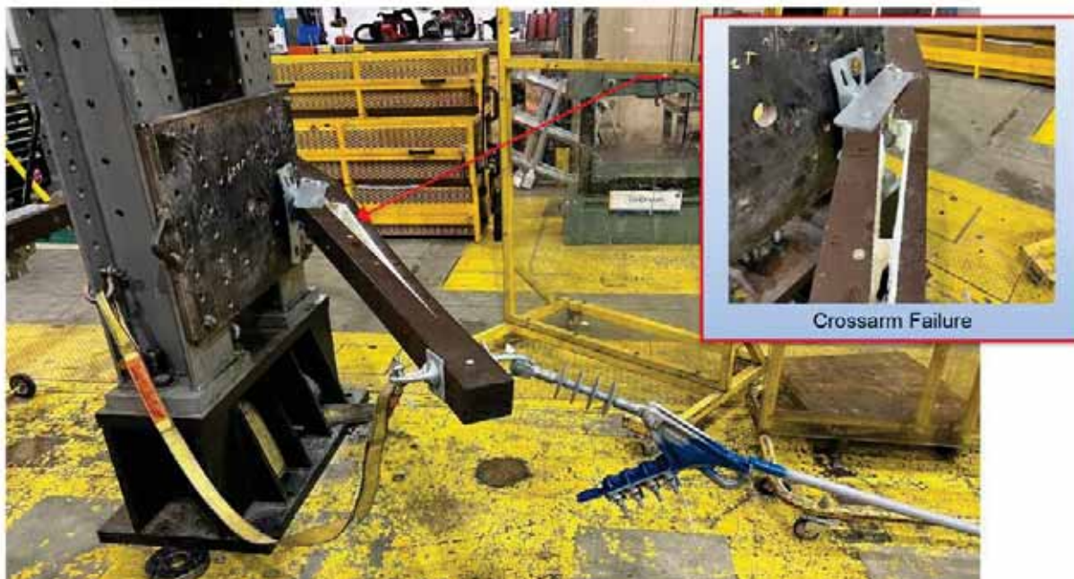
Figure E4. A representative post-test image showing splitting and failure of the composite cross-arm. 336.4 kcmil ACSR (30/7) with Type C dead-end shown.
