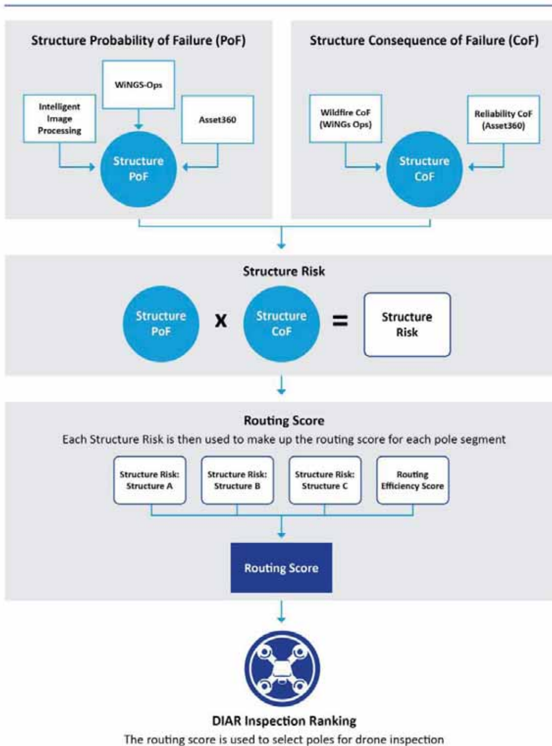
Figure 8-13: DIAR Inspection Prioritization Model
